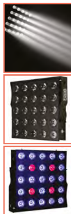
BEAM MATRIX5x5-RGBW 5x5 MATRIX effect, 25x 15W RGBW 4.5°beams + Artnet
